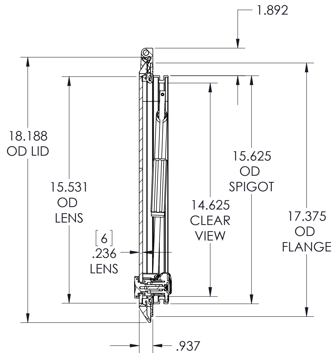
SECTION B-B
